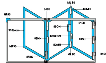
Diagram: Heavy Duty Side Hinge
